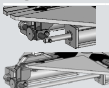
FLEX adjustable clamping system (increased clamping capacity 10" ÷ 27")
